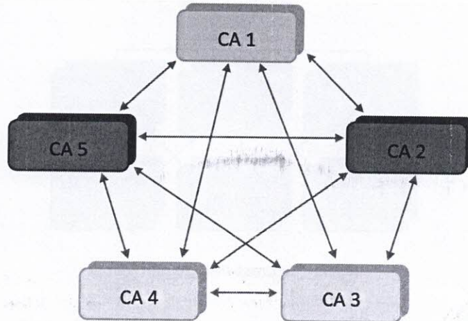
Figure F.2: Cross-Certification Model
