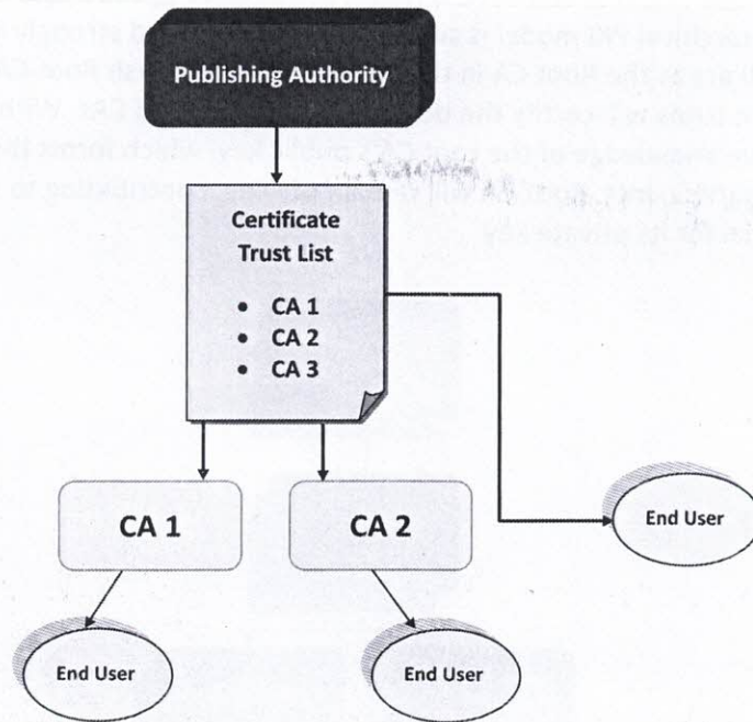
Figure F.5: CTL Model
